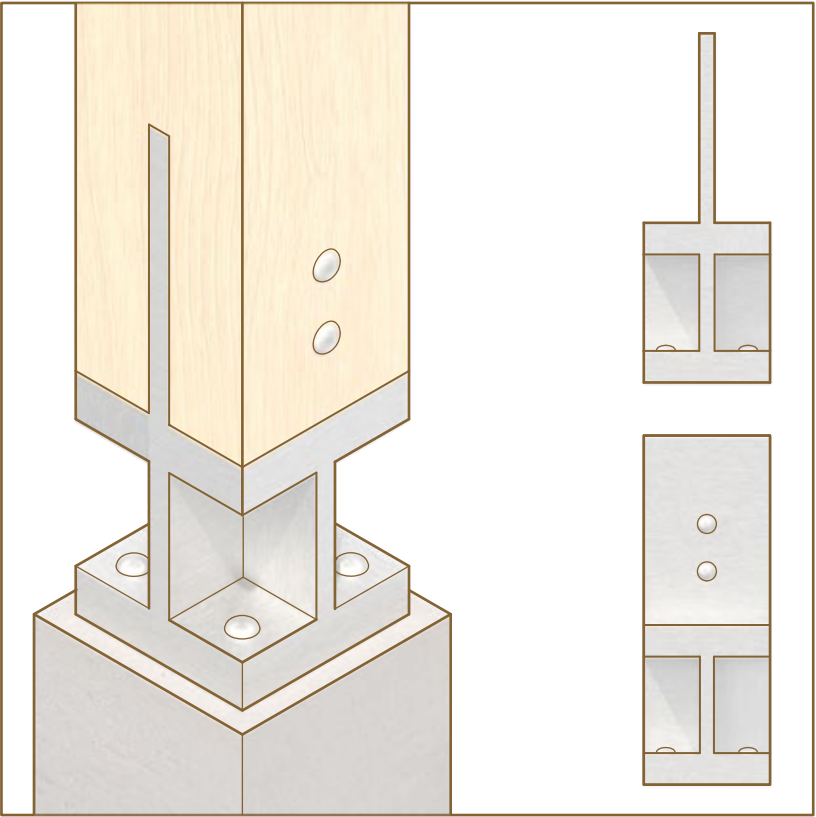
KNIFE PLATE CONNECTOR DETAIL
