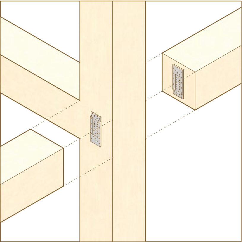
CONCEALED BEAM HANGER DETAIL
